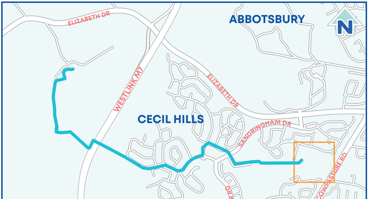
Pipeline route between Liverpool and Cecil Park Reservoirs
