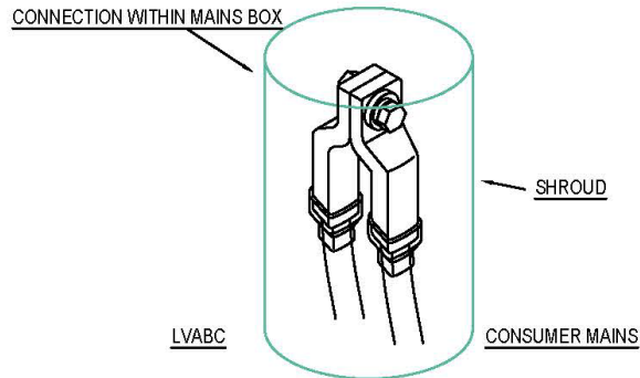
LVABC CONNECTION TO SINGLE CONSUMER MAINS
