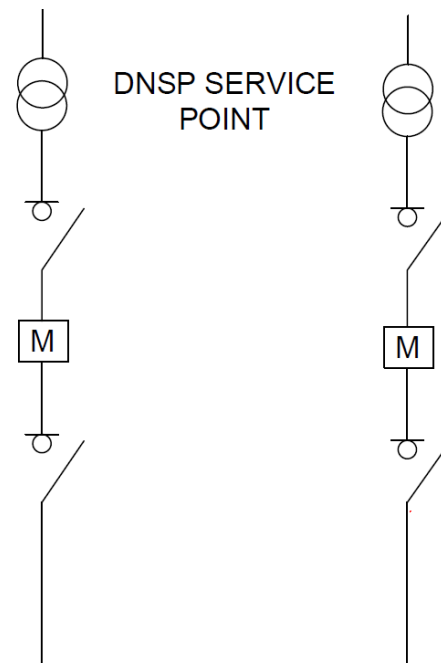
Figure 2 General arrangement of multiple DNSP service point with no bus-tie
