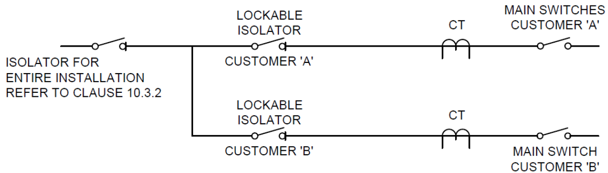
Figure 8: Typical CT Metering Arrangement for Multiple Customer
