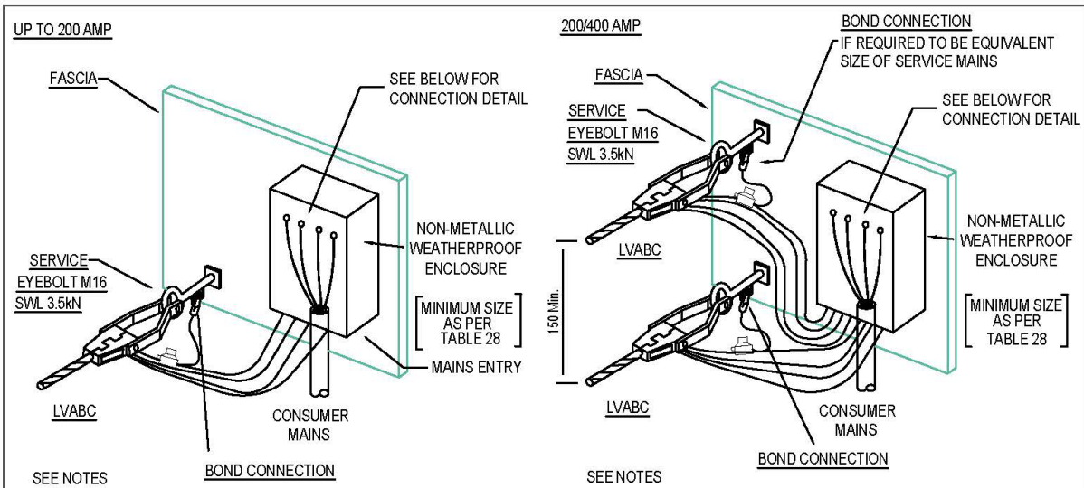
SINGLE SERVICE LINE CONNECTION DETAIL
