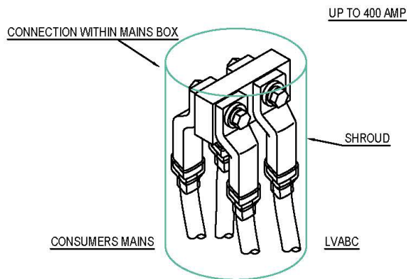
LVABC CONNECTION TO PARALLEL CONSUMER MAINS
