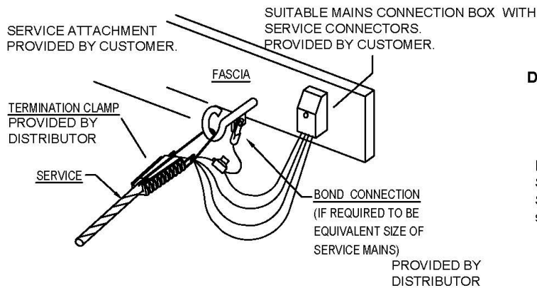
THREE PHASE SERVICE ARRANGEMENT SHOWN
