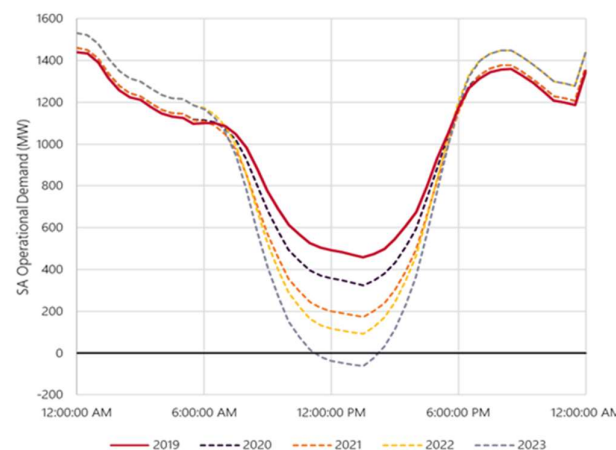
Figure 2 Effect on SA net operational demand from increasing solar PV generation
