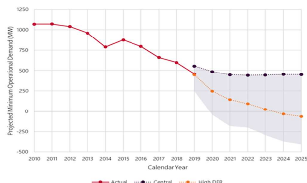
Figure 3 Minimum operational demand for SA
