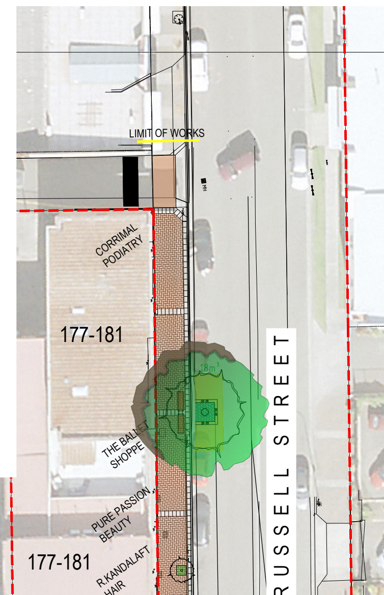
RUSSELL STREET TREE PLANTING Driveway crossing to be replaced with kerb and gutter - tree to be planted in parking lane in this location.
