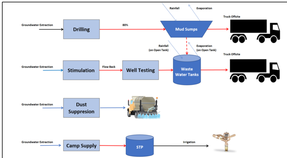
Figure 32: Site water management schematic
