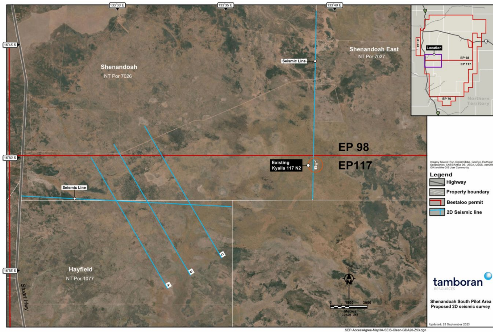
Figure 8: Proposed 2D seismic acquisition
