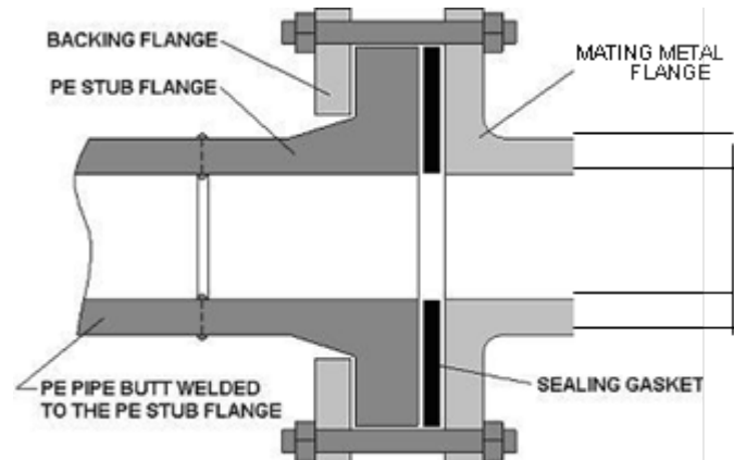
Figure 18: Typical flanged connection (source: APGA, 2019)
