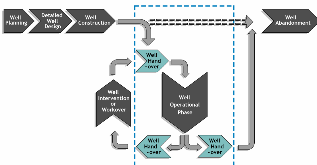
Figure 34: Well lifecycle with operational phase highlighted where well integrity monitoring is a key activity
