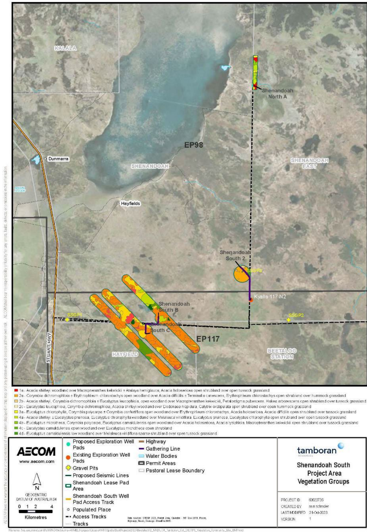
Figure 4: Vegetation communities for new sites
