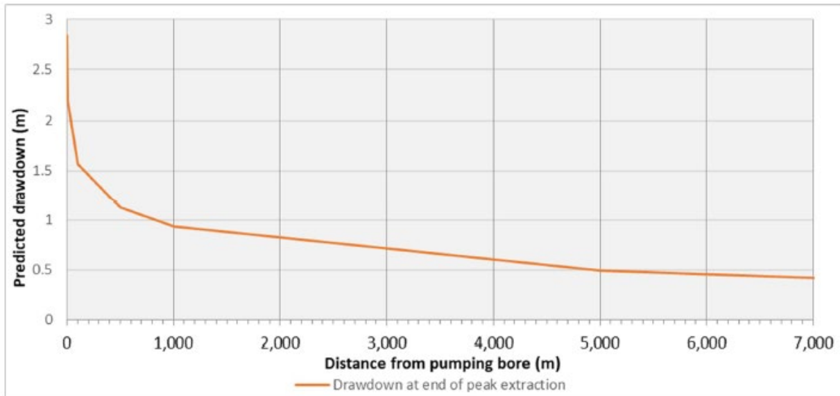
Figure 31: Modelled peak drawdown associated with anticipated future E&A water extraction take
