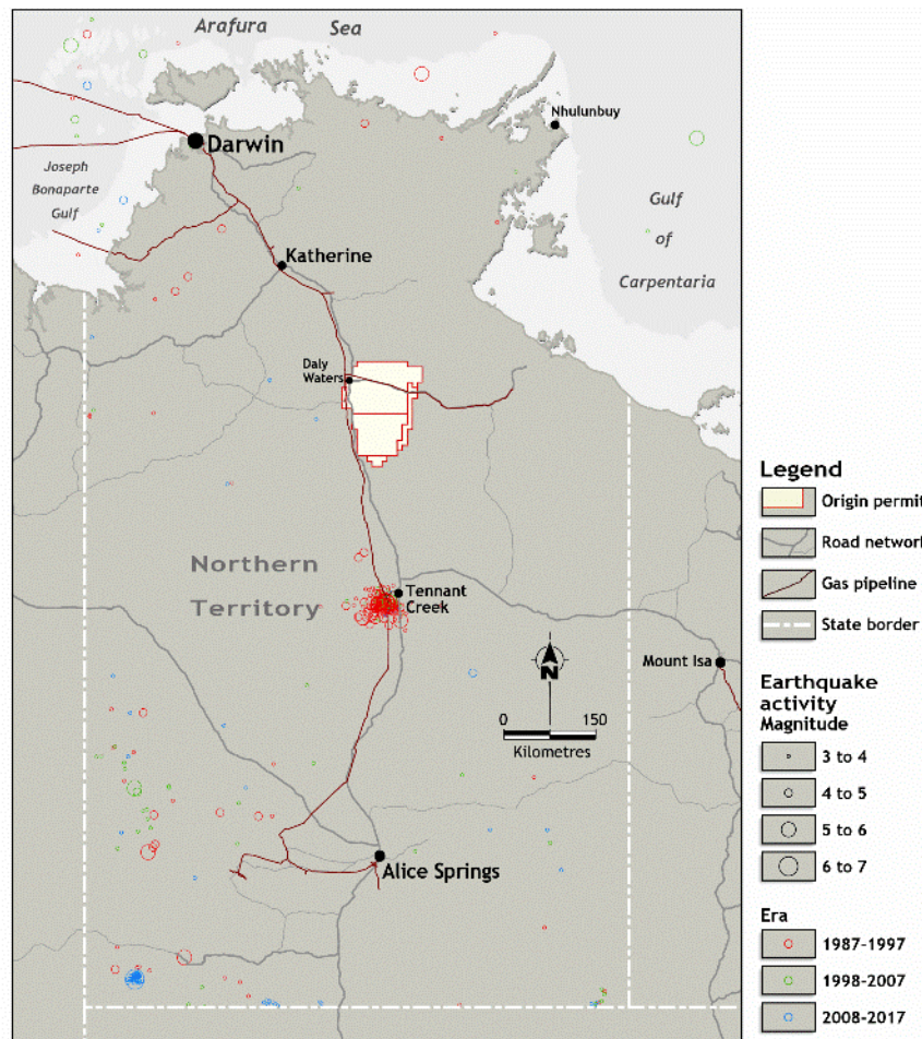
Figure 41: Earthquakes greater than magnitude 3 from 1987 to 2017 across the NT showing an absence of seismic activity in the Beetaloo area
