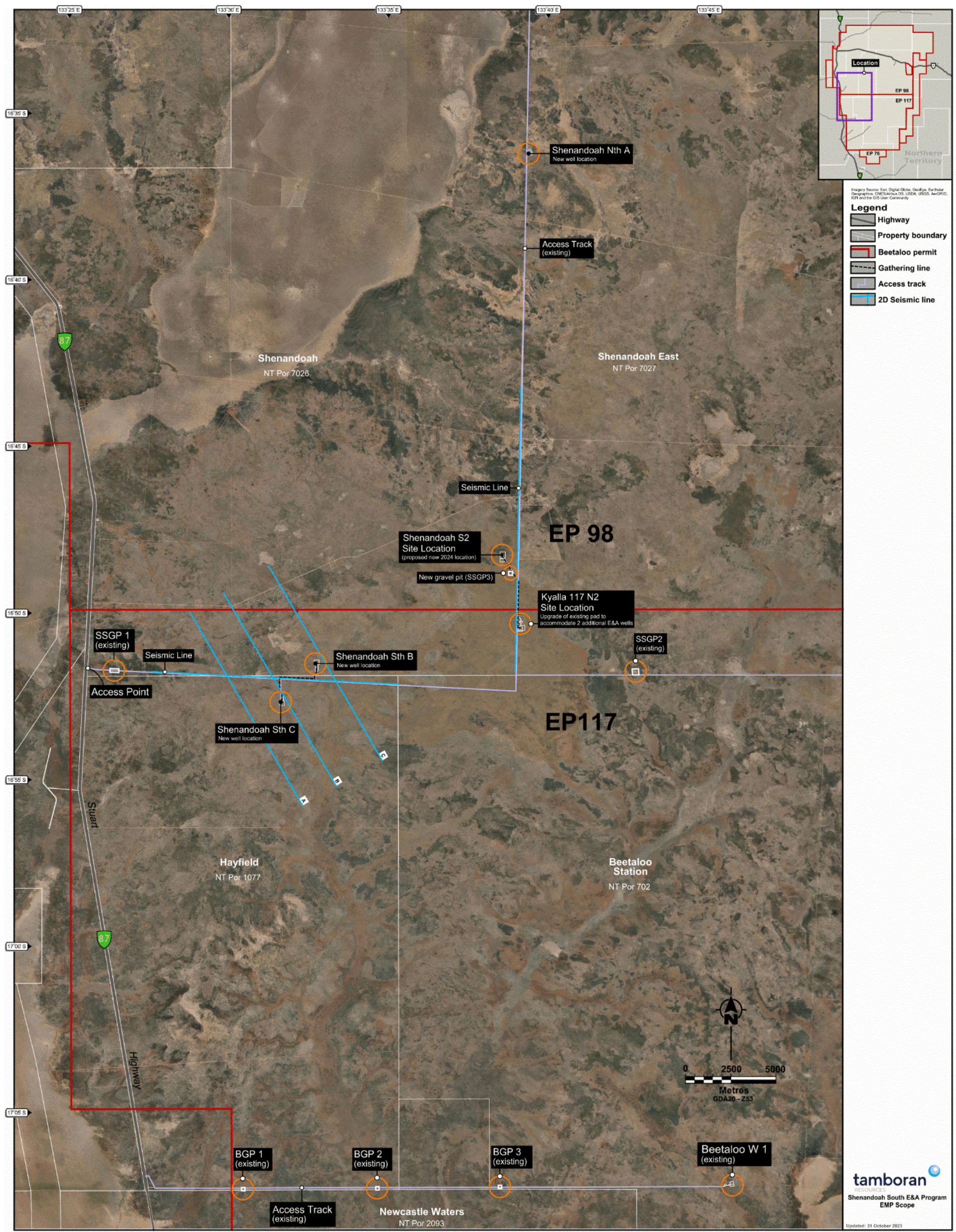
Figure 6: Location of all sites, associated infrastructure and the proposed 2D seismic program covered by this EMP
