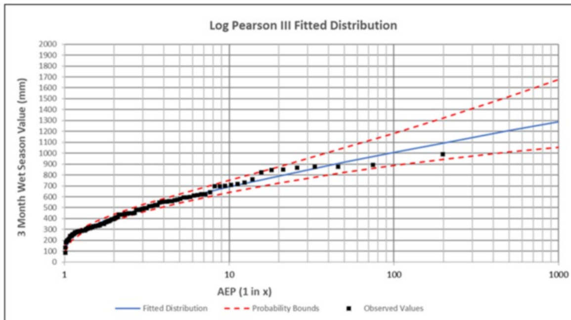
Figure 39: Log Pearson determination of 1:1000 wet season ARI
