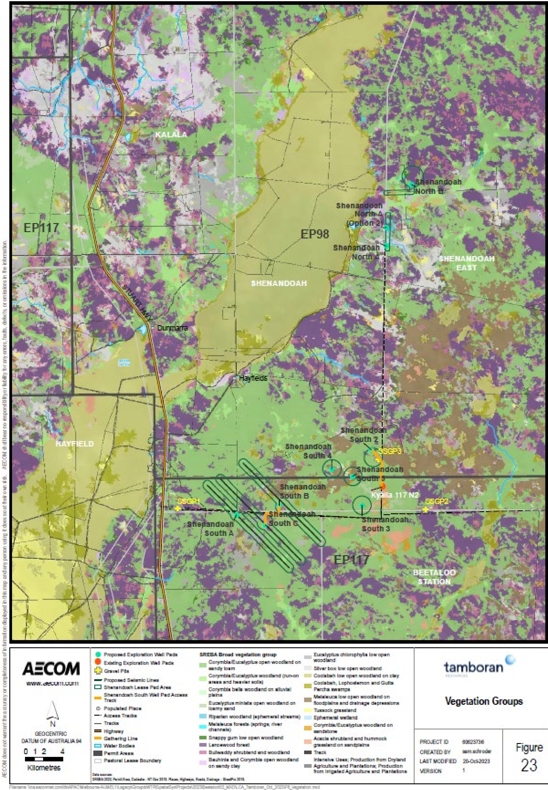
Figure 43: Shenandoah South E&A program SREBA vegetation community boundaries. Nb: this contains additional sites which were assessed during site selection that have not been progressed.
