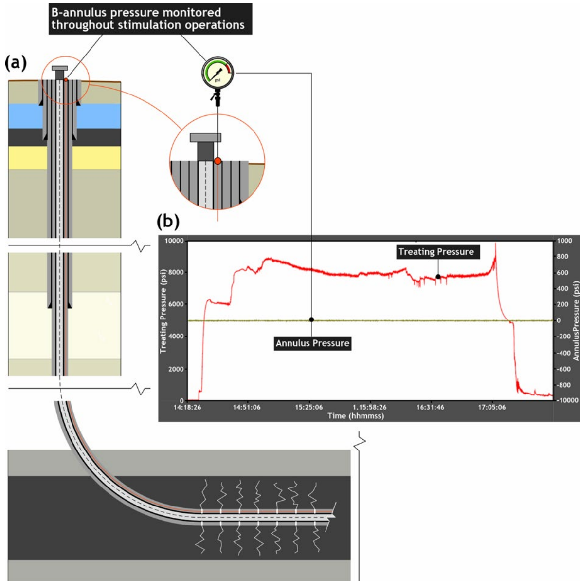
Figure 28: Well and wellhead schematic showing the "B Annulus" monitoring process, and an example from stage 1 of the observed pressure of the B Annulus (0 psi) while high-pressure HFS operations were underway
