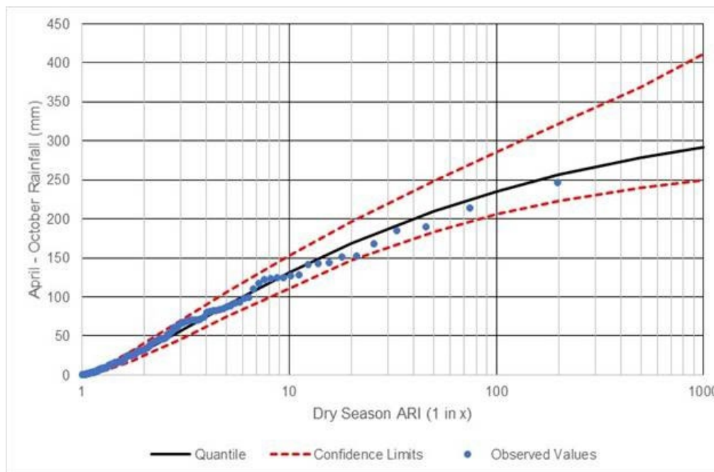
Figure 40: Log Pearson determination of 1:1000 dry season ARI
