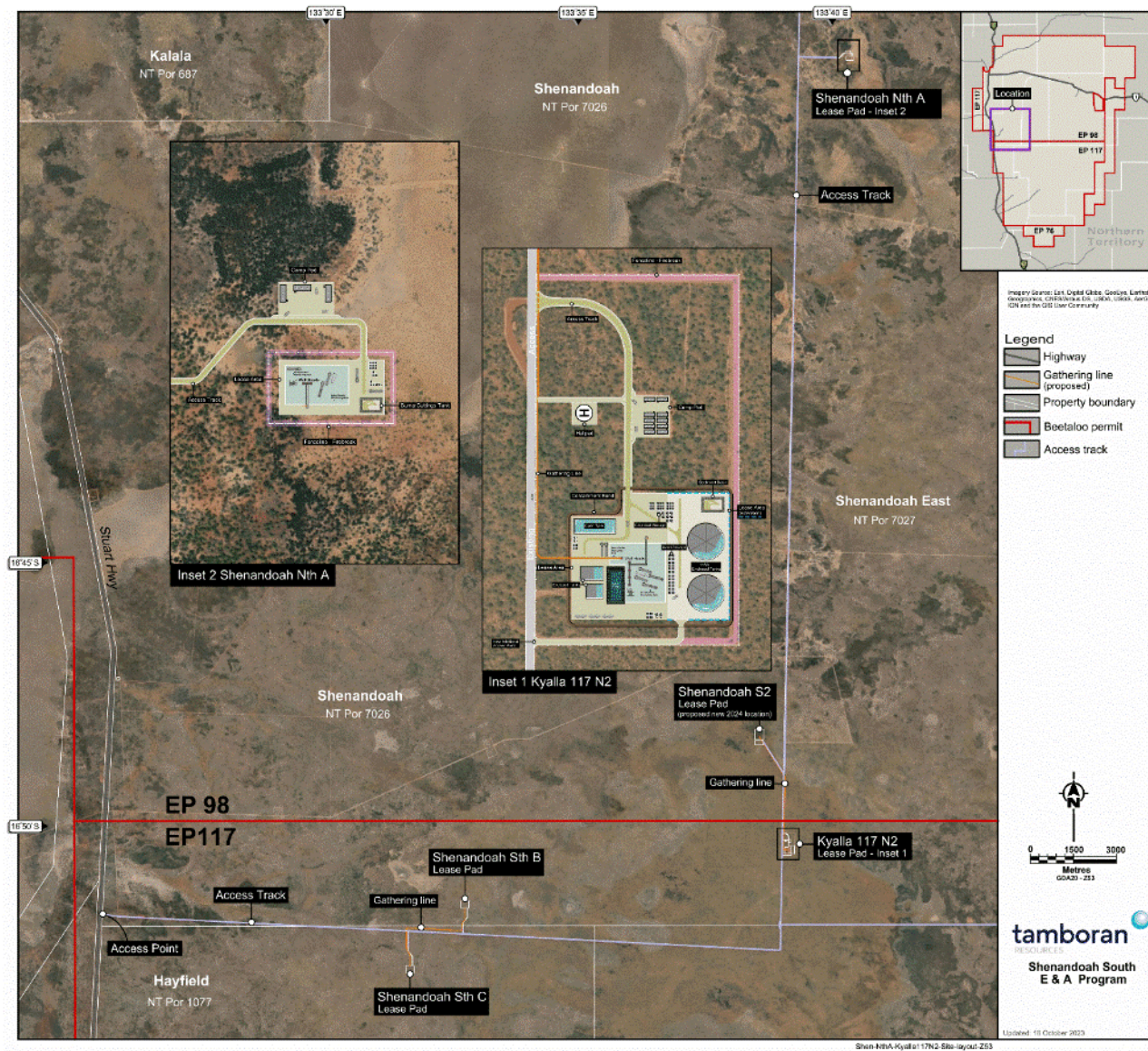
Figure 23: Generalised site layout for new E&A lease pad Shenandoah N A and existing Kyalla 117 N2, including increased lease pad
