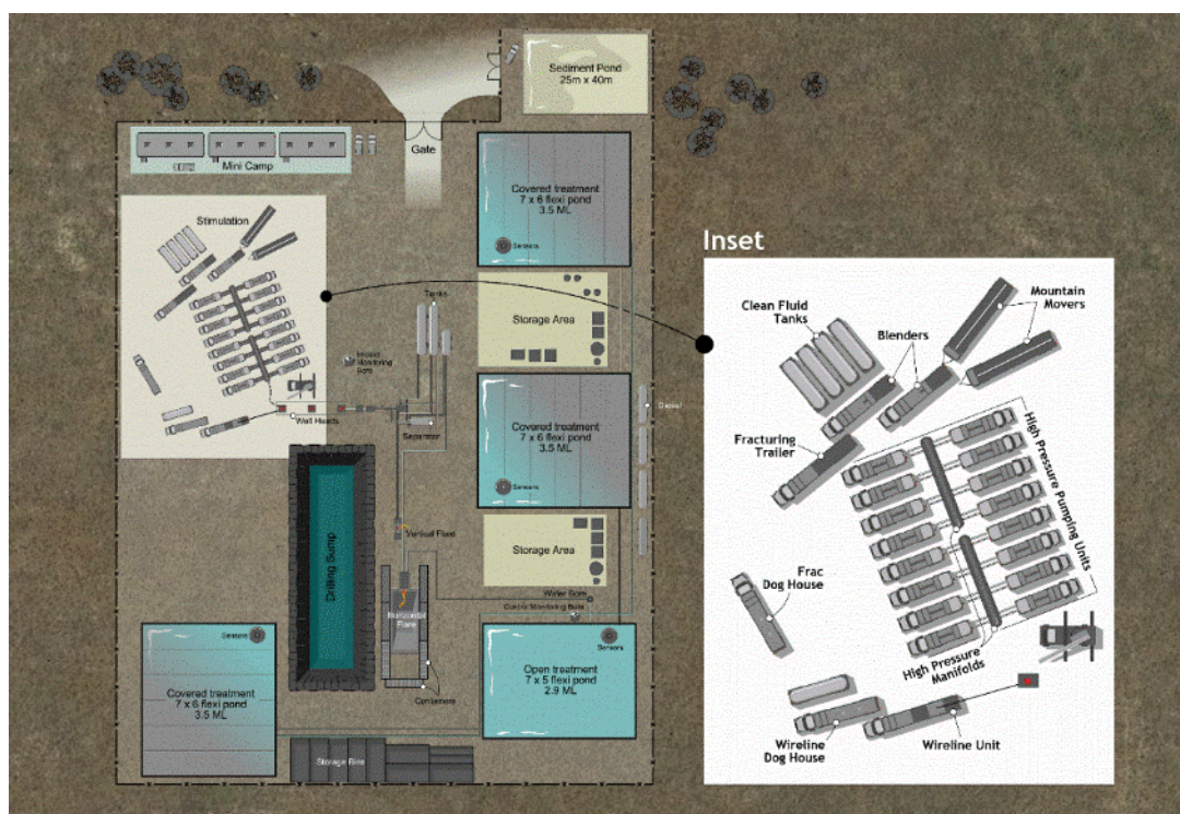
Figure 25: Indicative HFS spread used for each E&A well (NB: additional tanks will be installed where the frack spread is located during well test)
