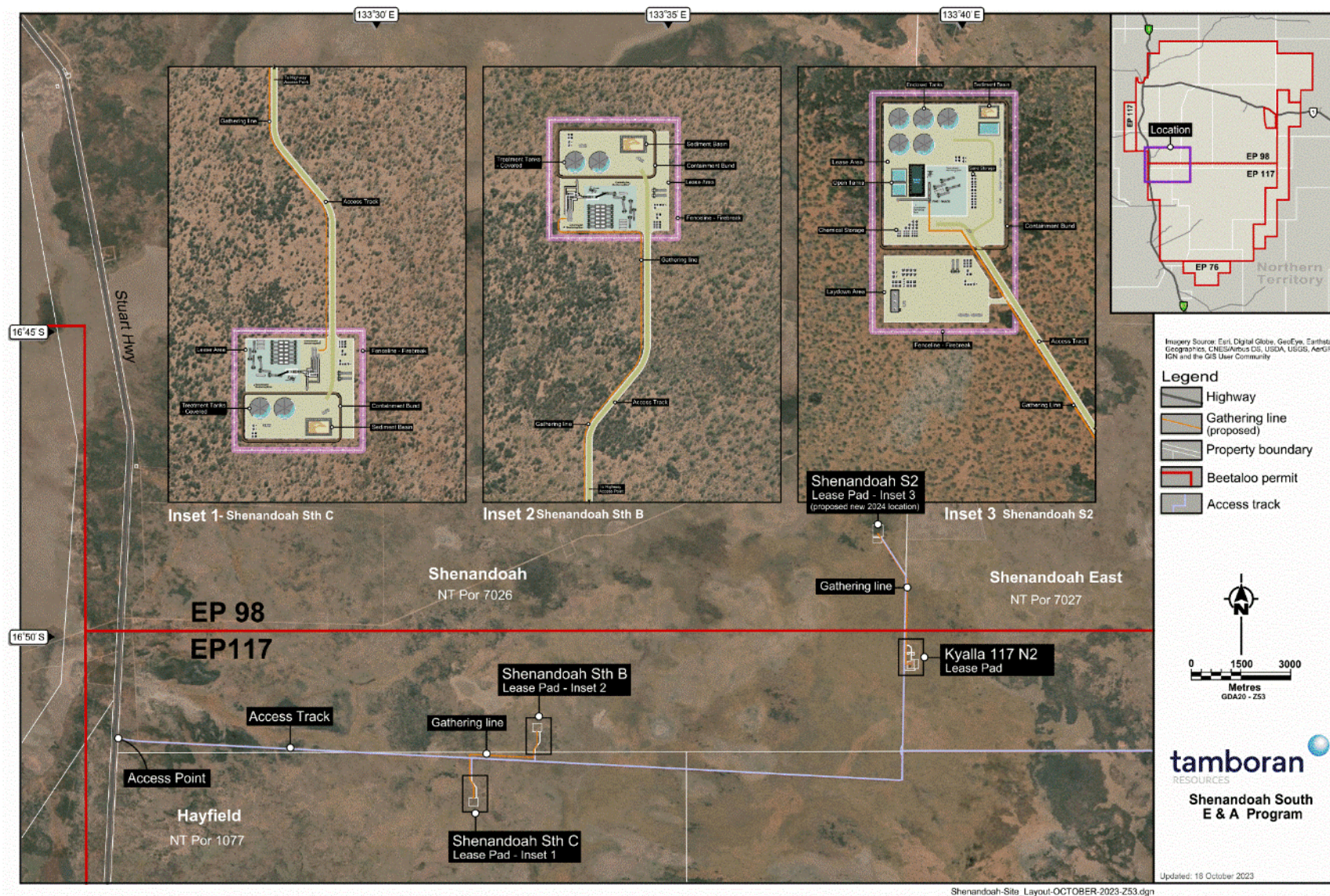
Figure 22: General site layout for new E&A lease pads – Shenandoah S2, S B and S C
