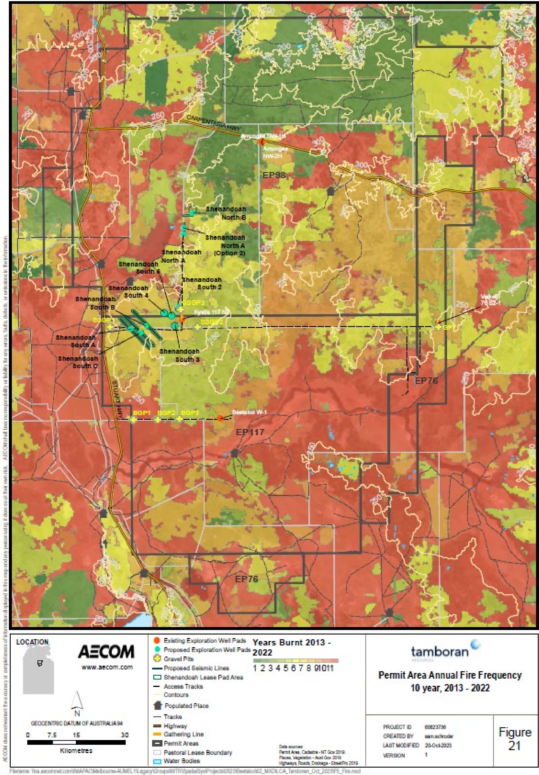
Figure 47: Fire frequency map . Nb: this contains additional sites which were assessed during site selection that have not been progressed.
