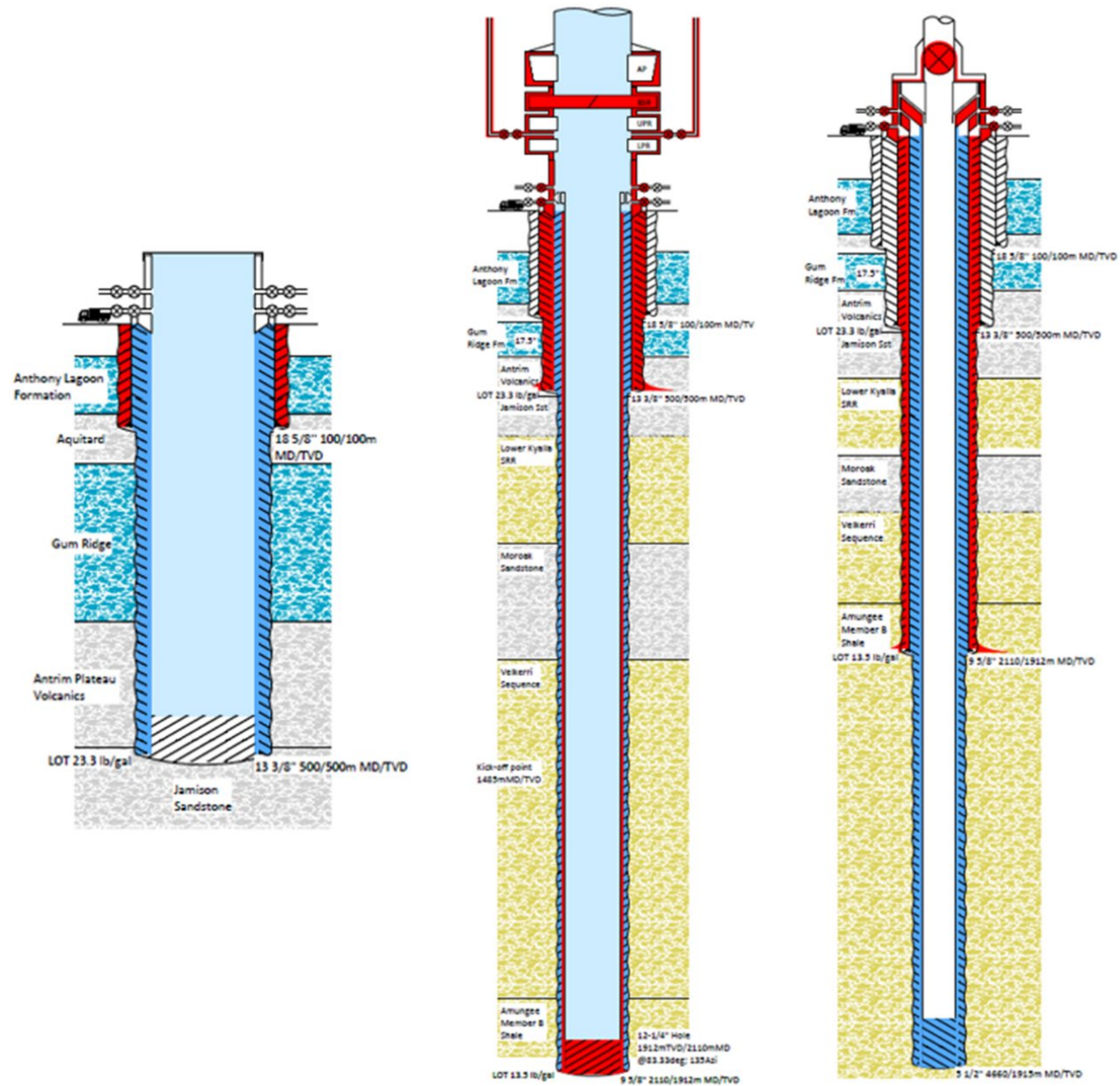
Figure 19: Typical well sections for the E&A wells – this includes the conductor and surface, intermediate and production casing strings of each exploration well
