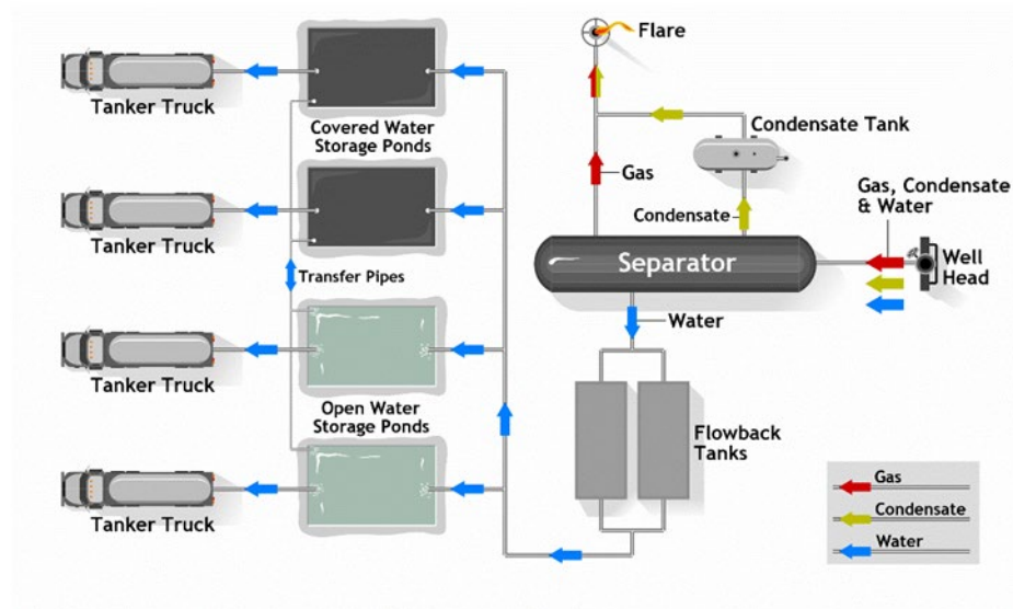
Figure 29: Sample well test schematic
