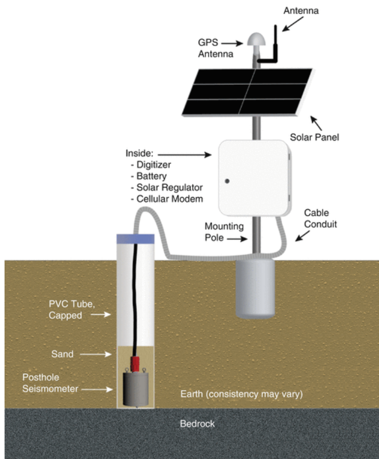
Figure 35: Seismic monitoring array to be set-up adjacent to selected exploration sites to monitor seismic activity
