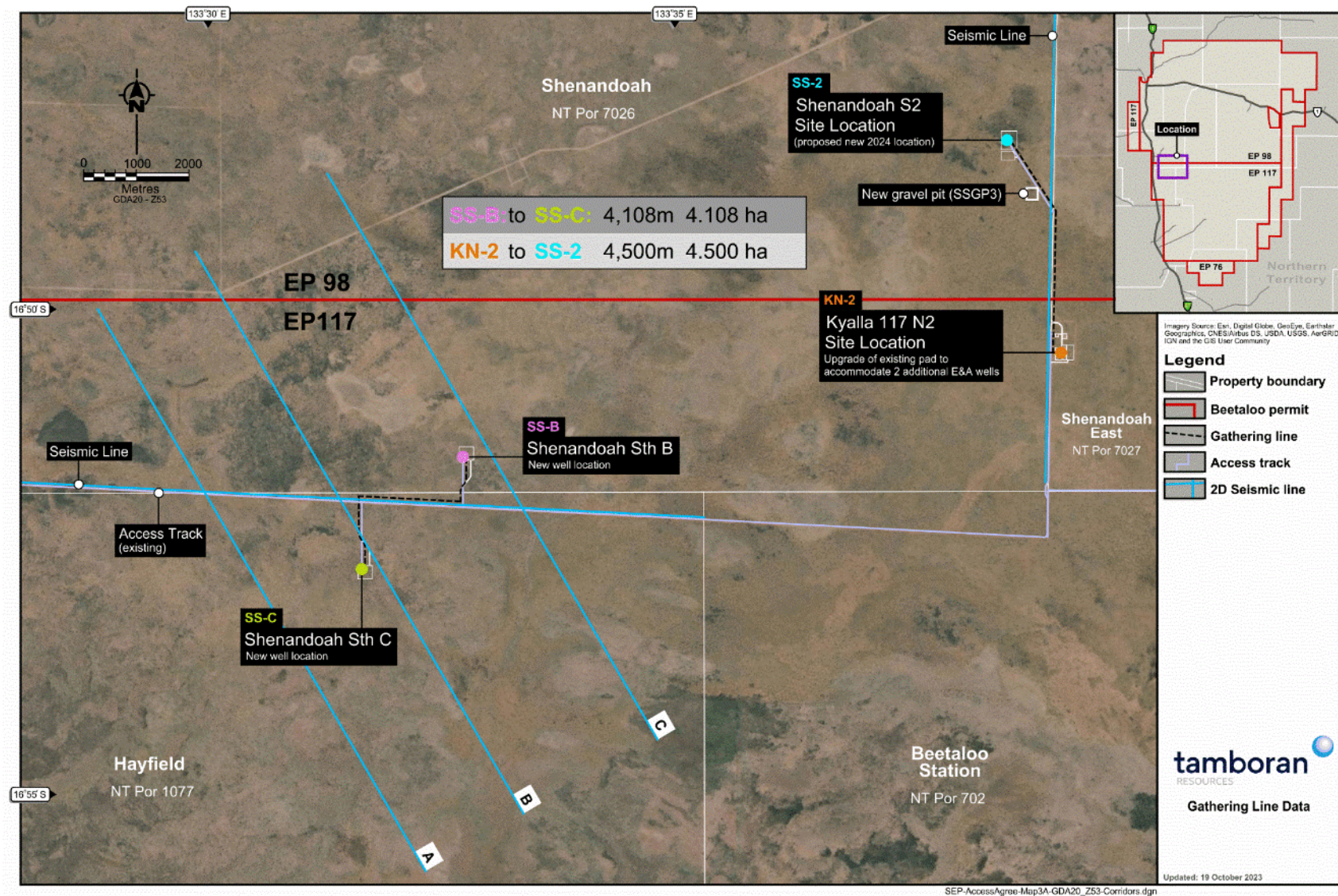
Figure 16: Gathering lines between the well sites
