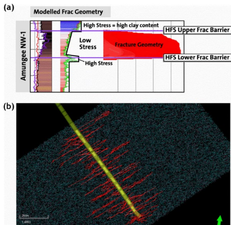
Figure 27: Example of visualised fracture geometry of Amungee NW-1
